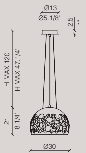
HOLE Ø30
