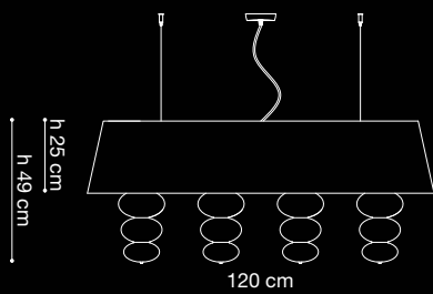
SO OVAL 120
